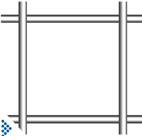
WM5050SS40/2.0 | Mesh Size 50.8mm Wire diameter 4.0mm
