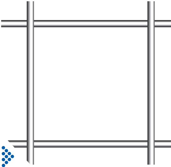
WM5050SS30/2.4 | Mesh Size 50.8mm Wire diameter 3.0mm
