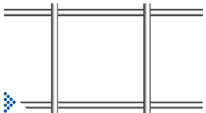
WM4040SS30/2.4 | Mesh Size 40mm Wire diameter 3.0mm
