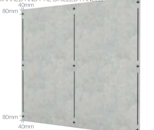
FIGURE 4 PRE MARKED AND PRE DRILLED PANELS
