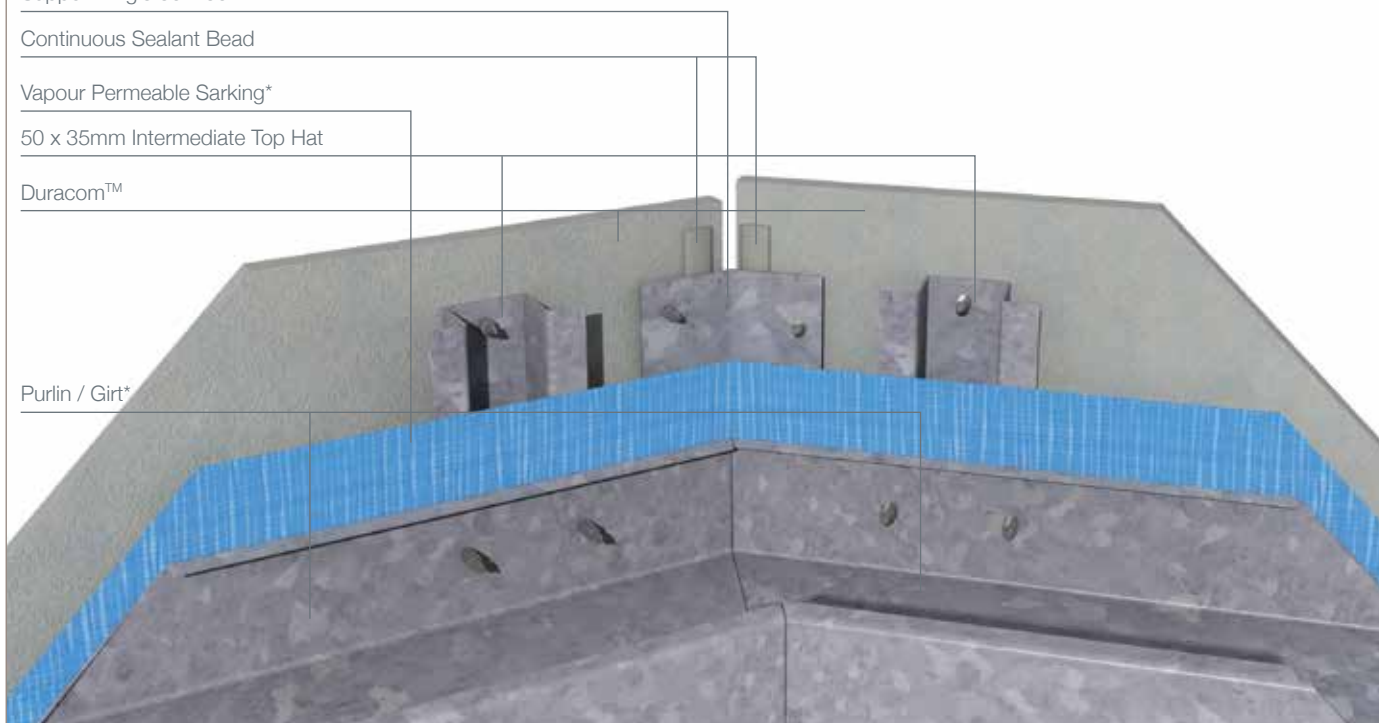
FIGURE 19 ANGLED INTERNAL CORNER
