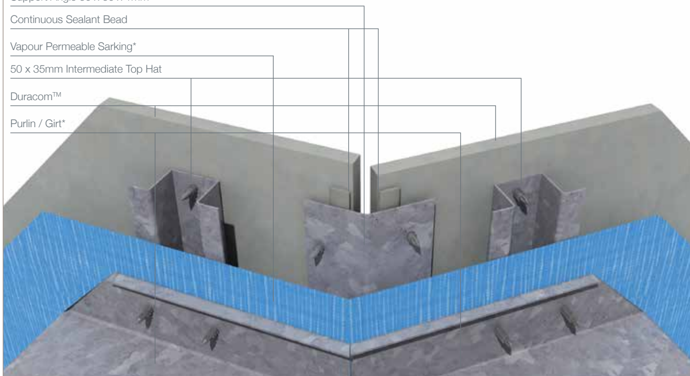
FIGURE 19 ANGLED INTERNAL CORNER
