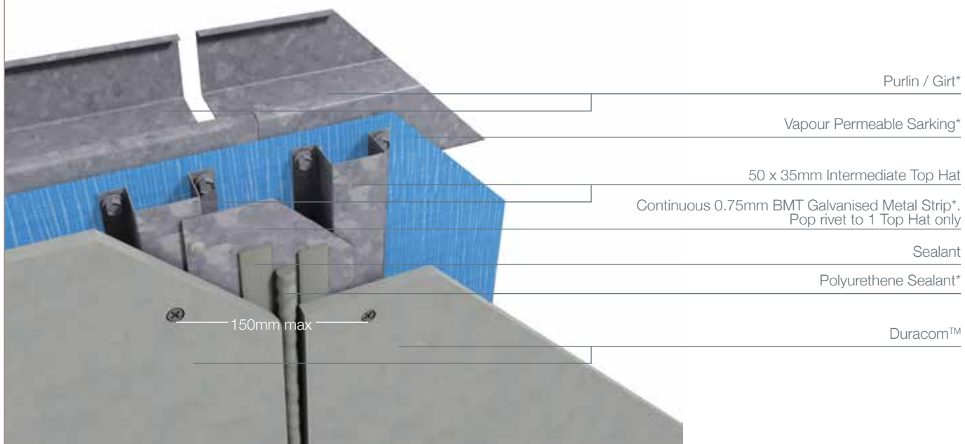
FIGURE 25 VERTICAL CONTROL JOINT
