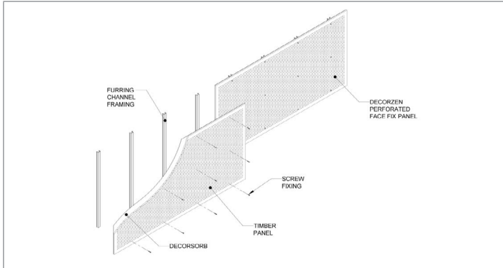
Wall & Ceiling Face Fixing
