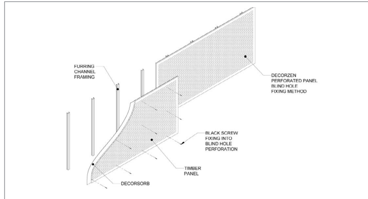
Wall & Ceiling Blind Hole
