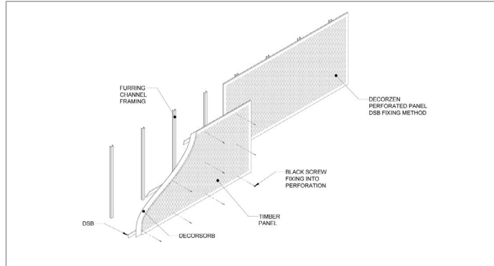
Wall & Ceiling DSB Fixing
