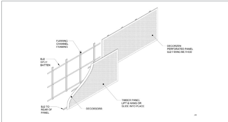
Wall BJ2 Fixing
